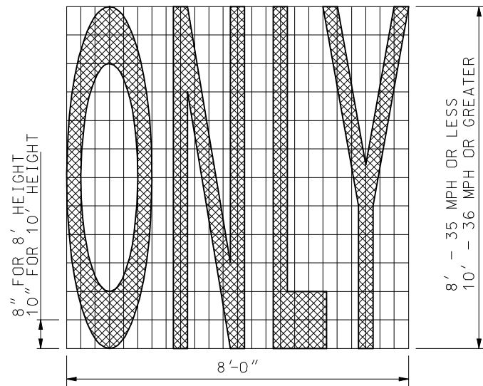
WORD MARKING ELONGATED WORD & SYMBOL
