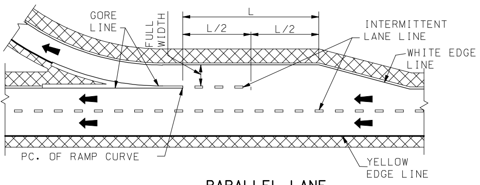
PARALLEL LANE
