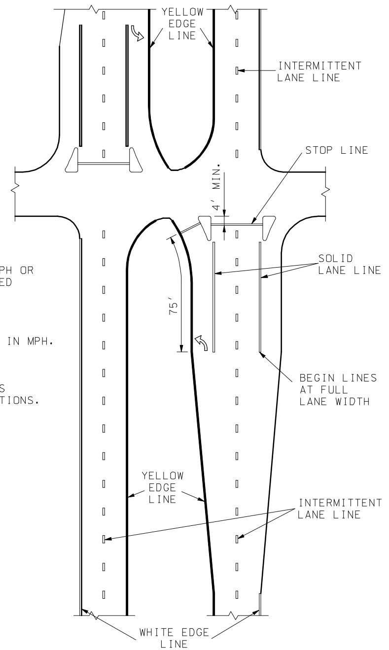
SIGNALIZED GRADE INTERSECTION MARKING
