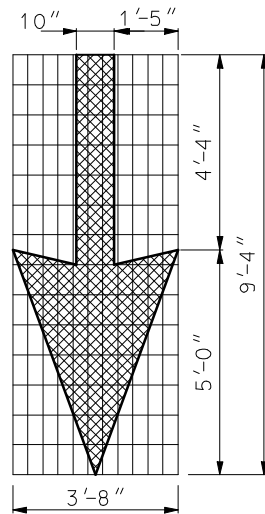
ARROW MARKINGS
