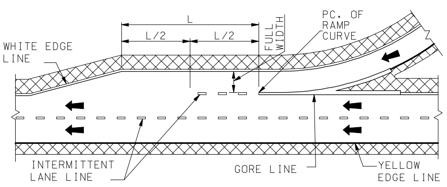
PARALLEL LANE
