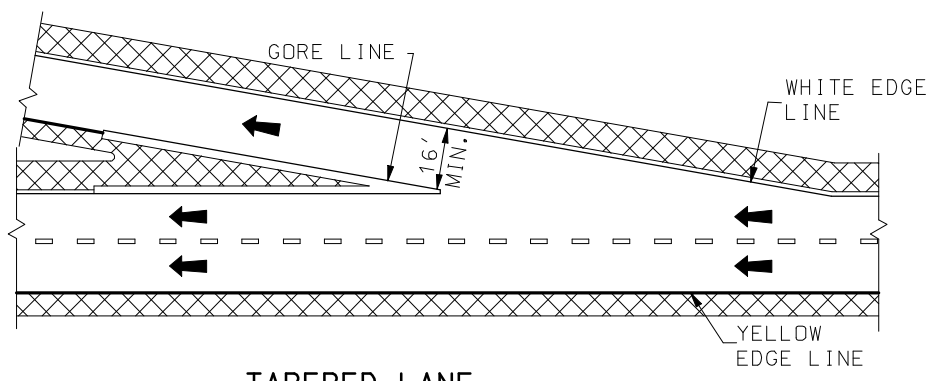
TAPERED LANE
