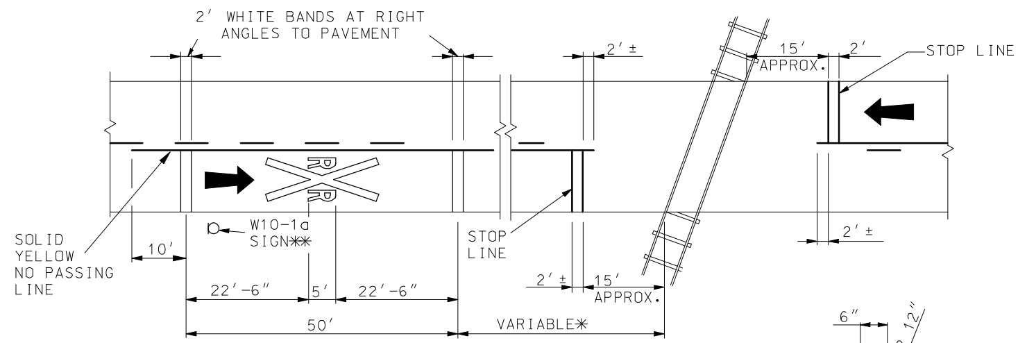
PAVEMENT DETAIL
