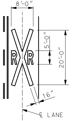
SYMBOL DETAIL
