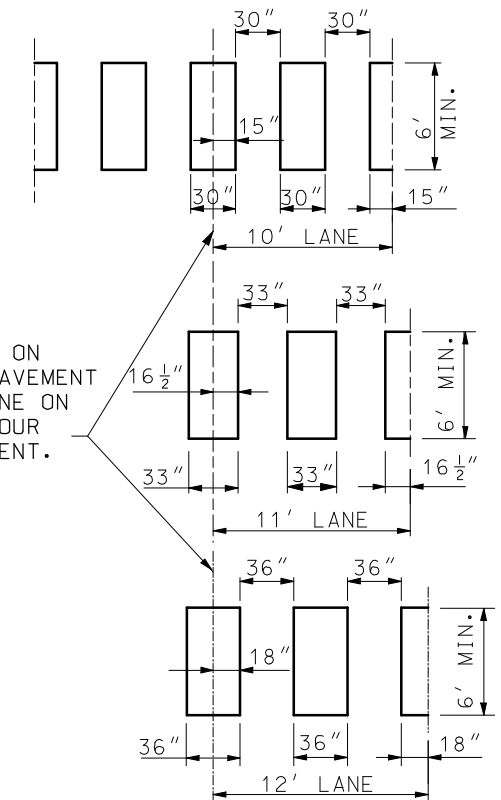
WHITE MIDBLOCK (ZEBRA)
