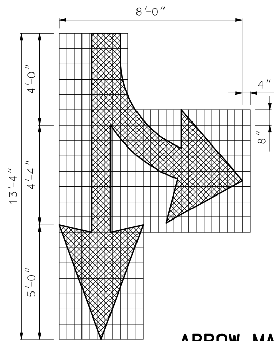
ARROW MARKINGS
