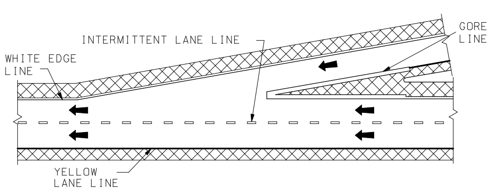
TAPERED LANE
