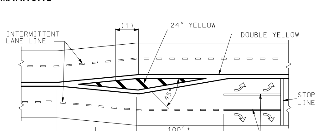
OFFSET BOTH LANES
