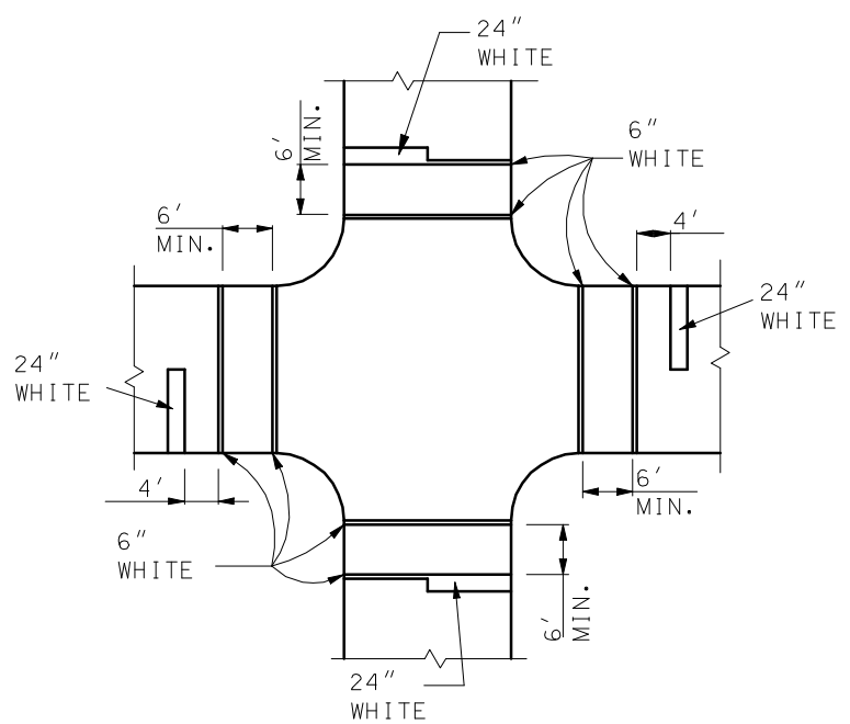
SOLID WHITE PEDESTRIAN CROSSWALK
